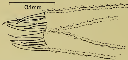
TEXT-FIG. 15.— Baccalareus verrucosus sp. nov. Caudal fork.
